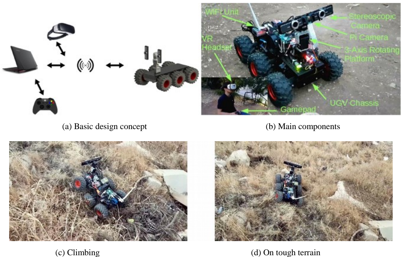
Figure 2. The UGV.
